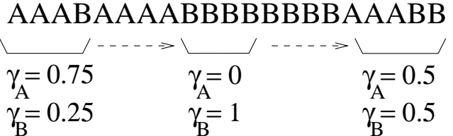
Figure 7: Illustration of the Sliding Window Method.
